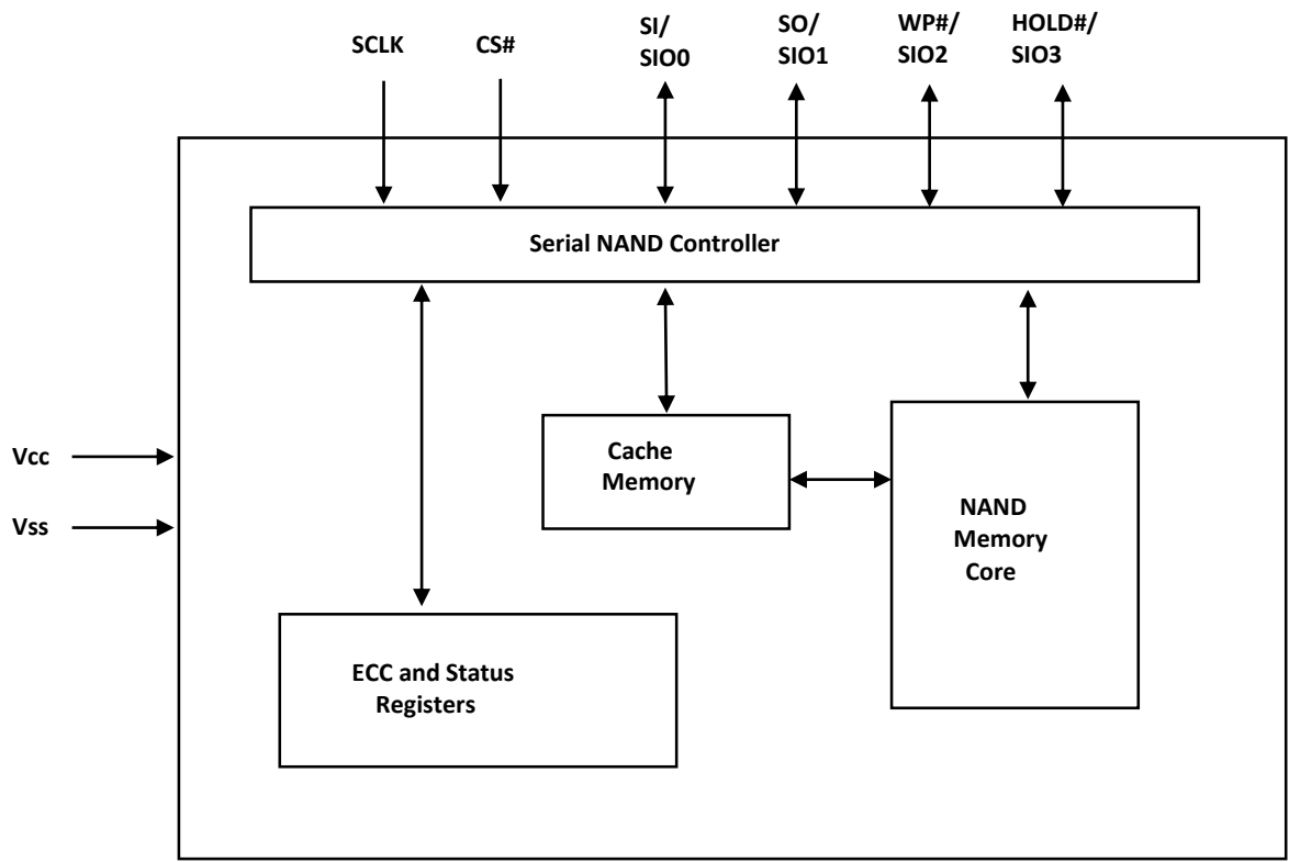
Figure 1.2 Block Description
