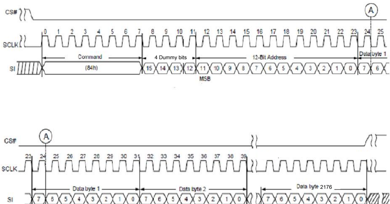
Figure 3.13 Program Load Random Data (84h)
