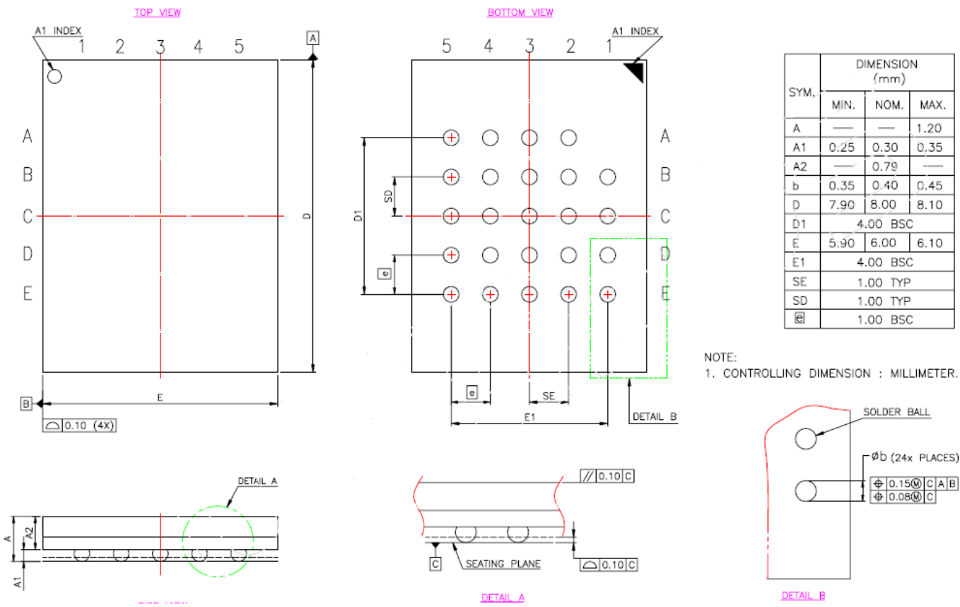
Figure 6.4 BGA24(5x5 Ball Array)
