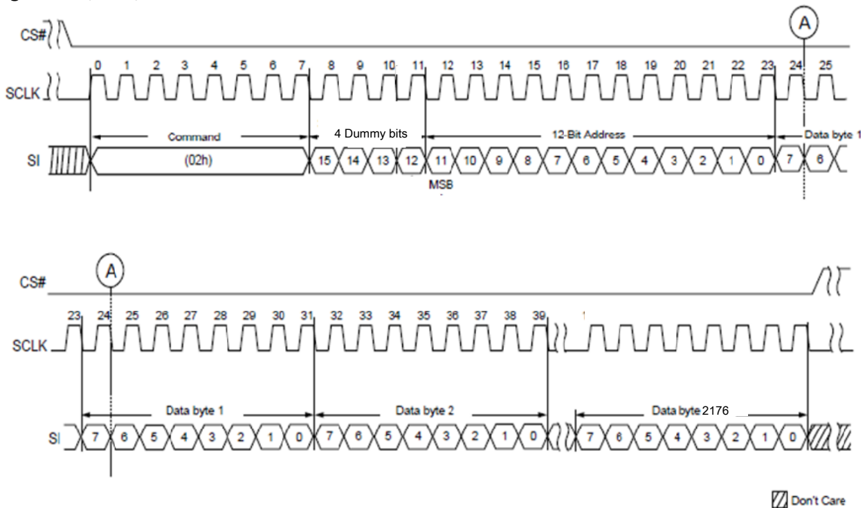
Figure 3.10 Program Load (02h)
