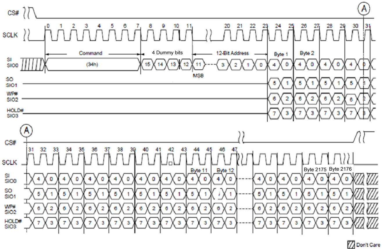
Figure 3.14 Program Load Random Data x4 (34h)
