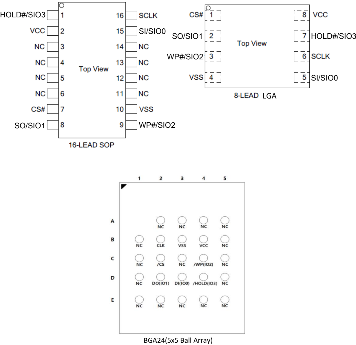
Figure 6.1 Pin Configuration
