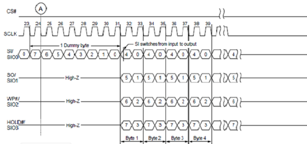
Figure 3.8 Read From Cache x4
