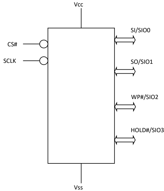
Figure 1.1 Logic Diagram
