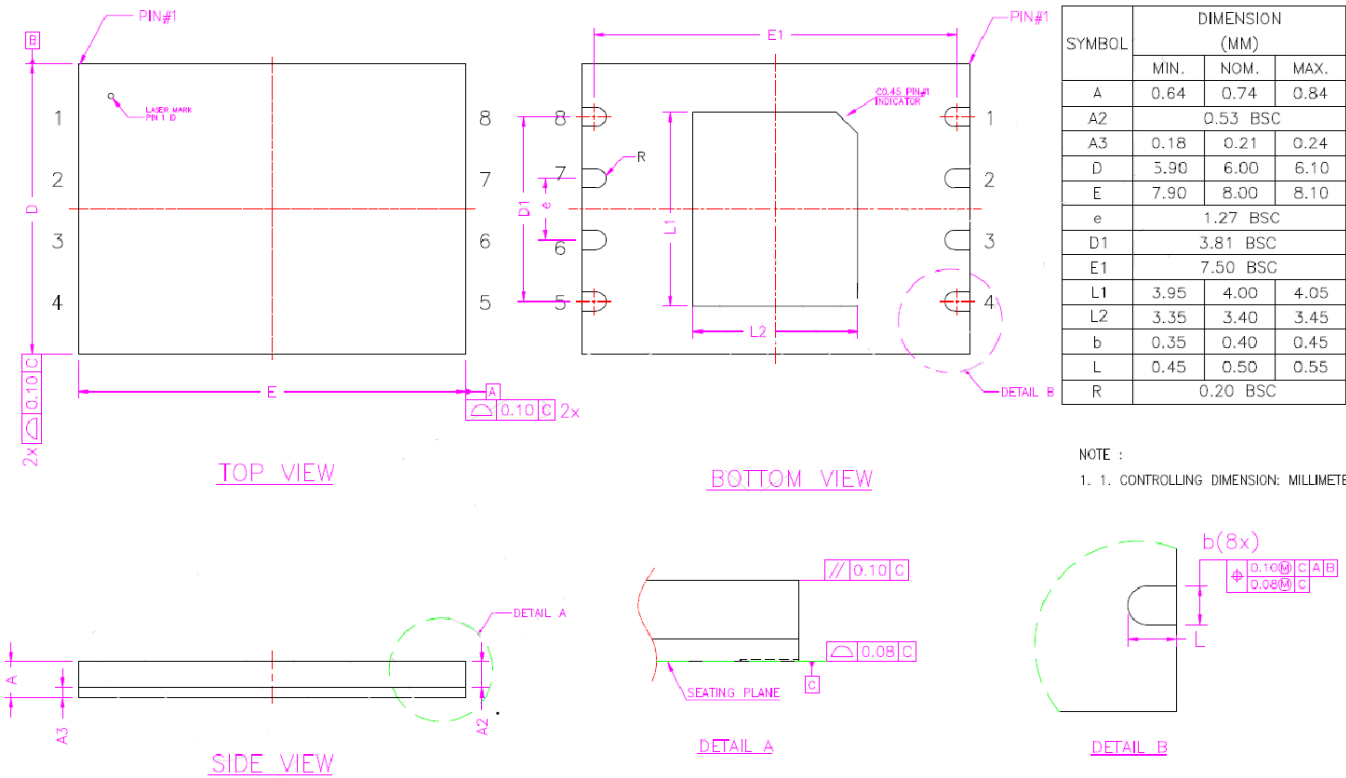
Figure 6.2 LGA (8*6mm)
